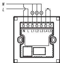
1-gang/2-gang/3-gang light panel+1-gang external linkage
