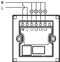
1-gang/2-gang/3-gang/4-gang light panel
